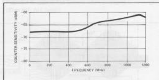
Figure 4-2. Typical 8901A counter sensitivity when manually tuned.
