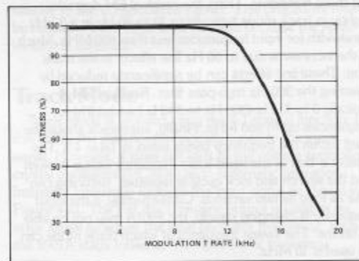
Figure 4-27. Typical 15 kHz low-pass filter response.
