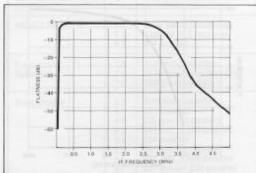
Figure 4-23. 1.5 MHz IF filter characteristic.
