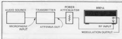
Figure 2-1. Transmitter test setup.
