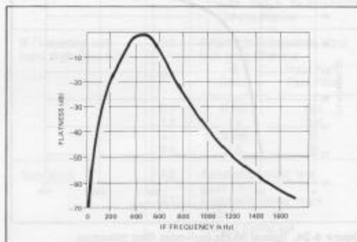
Figure 4-22. 455 kHz IF filter characteristic.
