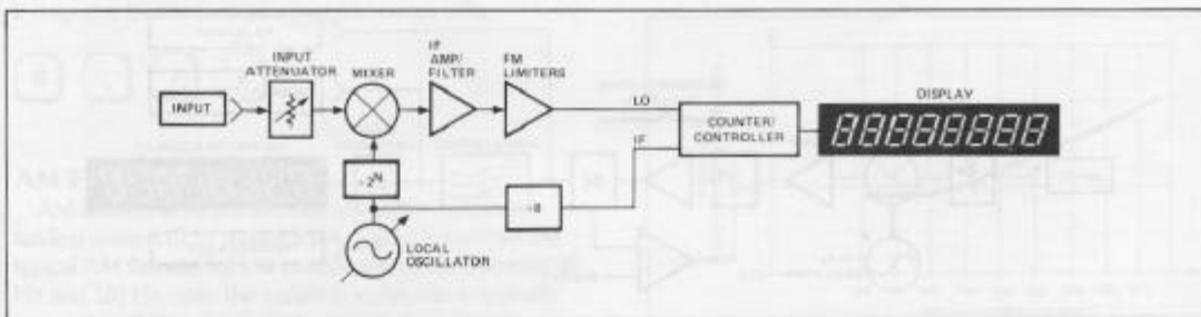
Figure 4-1. Input frequency measurement block diagram.
