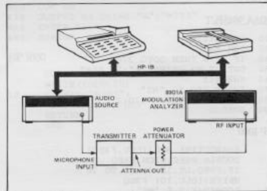
Figure 6-8. Automatic transmitter test equipment setup.
