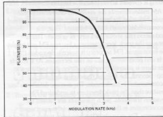
Figure 4-26. Typical 3 kHz low-pass filter response.
