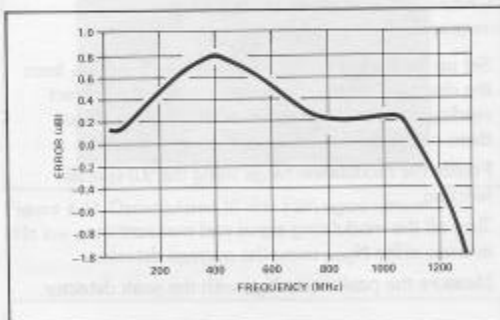
Figure 4-17. Typical 8901A RF level accuracy.
