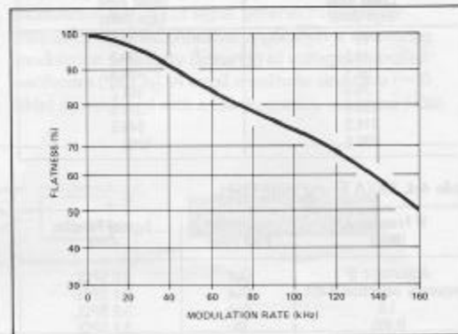
Figure 4-28. Typical >20 kHz low-pass filter response.
