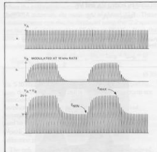
Figure 5-2. Forming the AM calibrator signal.
