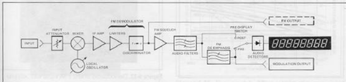
Figure 4-7. FM measurement block diagram.
