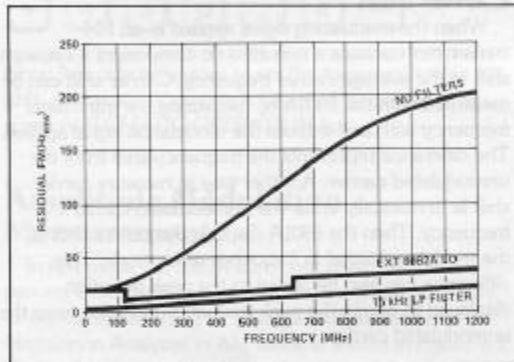
Figure 4-8. Typical 8901A residual FM.
