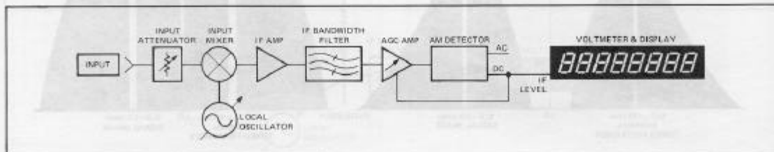
Figure 4-20. IF level measurement block diagram.
