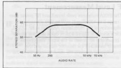
Figure 4-14. Typical 8901A stereo separation.
