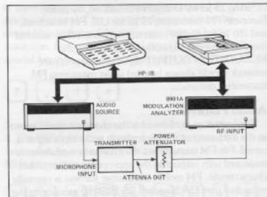
Figure 2-3. Automated FM transmitter testing
