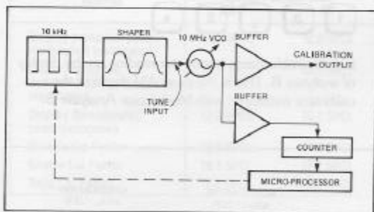
Figure 5-5. FM calibrator block diagram.
