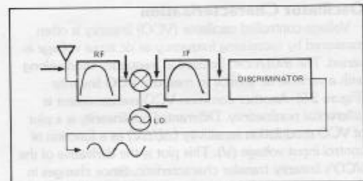
Figure 2-8. FM receiver design using the 8901A.
