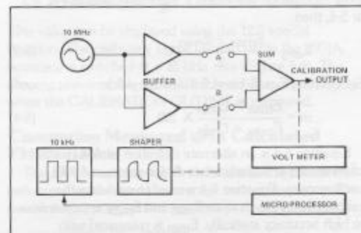
Figure 5-1. AM calibrator block diagram.
