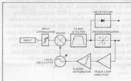
Figure 4-21. Track mode block diagram.
