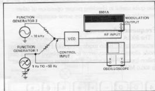
Figure 2-6. Equipment setup to measure real time VCO modulation sensitivity.
