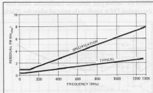
Figure 4-9. 8901A residual FM (50 Hz to 3 kHz BW).
