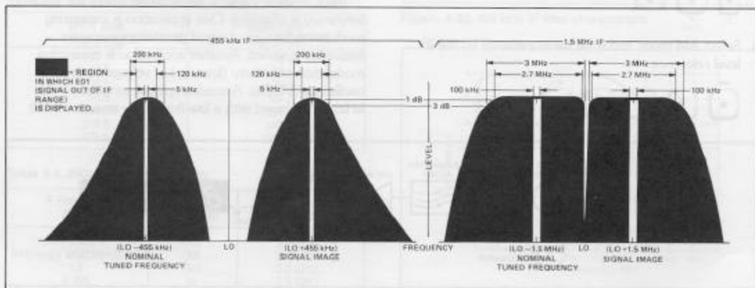
Figure 4-19. Typical 8901A IF bandwidth characteristics.
