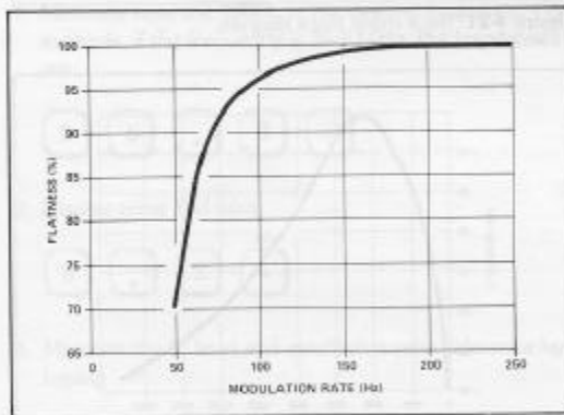
Figure 4-24. Typical 50 Hz high-pass filter response.
