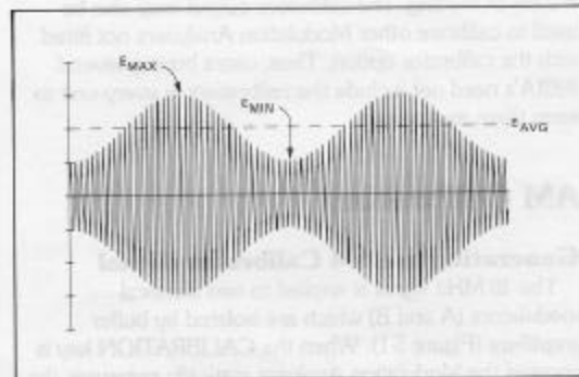
Figure 5-4. RF carrier modulated with 50% AM.
