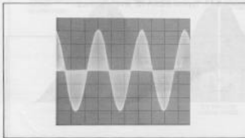
Figure 4-13. Demodulated 15 kHz FM stereo test signal.
