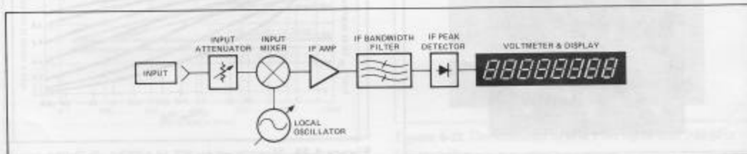
Figure 4-18. Tuned RF level measurement block diagram.
