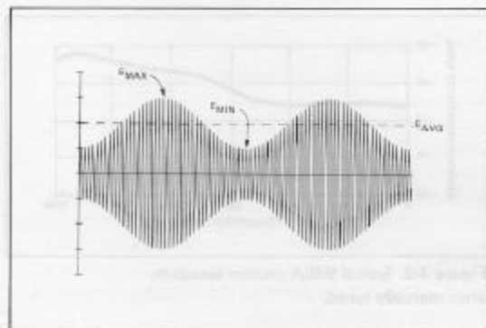
Figure 4-4. RF carrier modulated with 50% AM.
