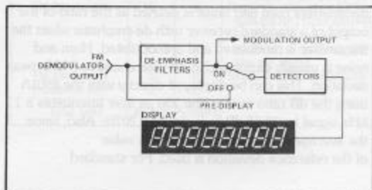
Figure 2-2. 8901A PRE-DISPLAY de-emphasis mode.
