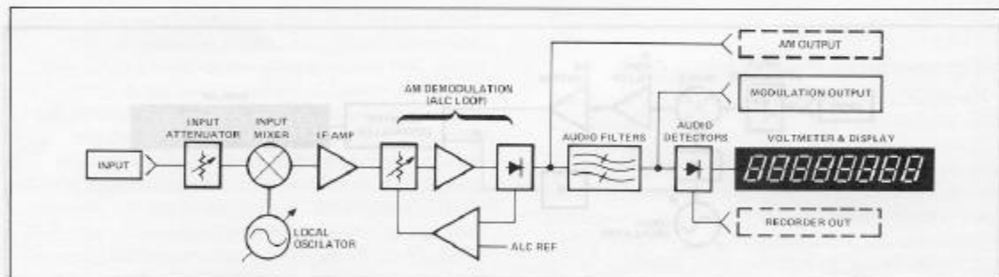
Figure 4-3. AM measurement block diagram.
